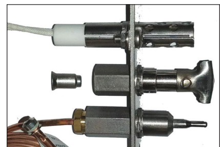
Figure 9.3 – Cleaning pilot orifice
