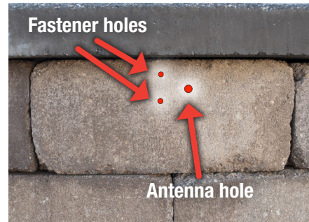
Figure 6.2 – Plot the hole locations
