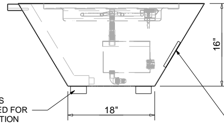
ELECTRONIC IGNITION OPTION
