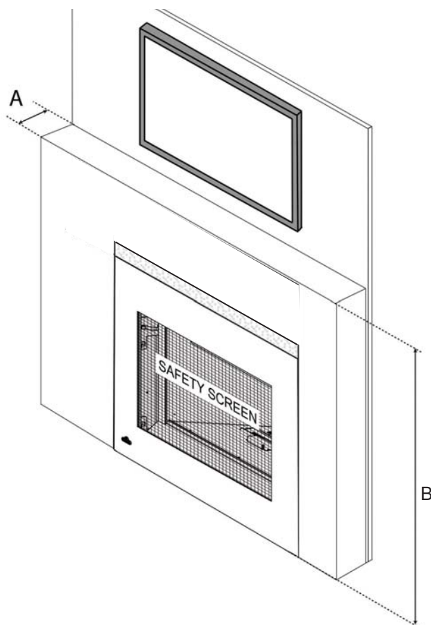
CLEARANCES CHART
